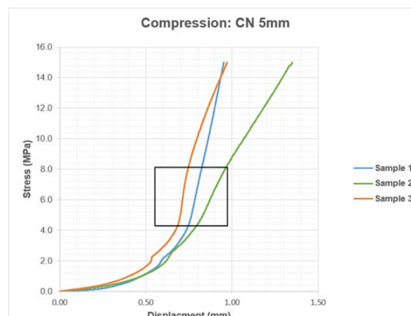
Figure 1 – Illustration of the Area the E-modulus was Calculated
